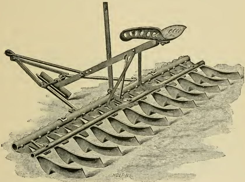
ACME HARROW.
